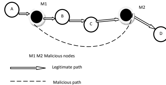
Figure 1. Wormhole Scenario
